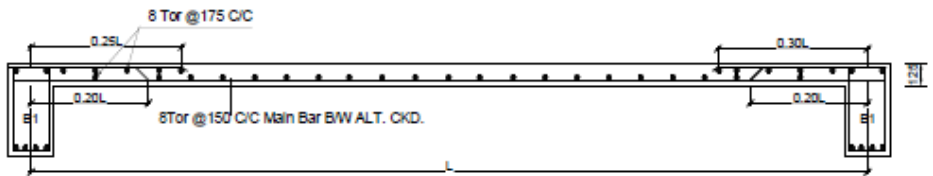
Fig 4.18 R.C.C SLAB
