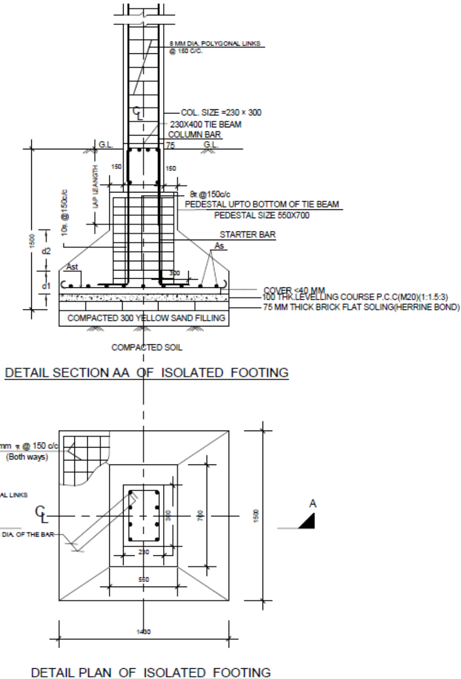
Fig 4.15 R.C.C Column Footing
