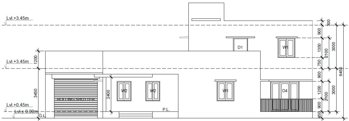
Fig 4.5 Elevation
