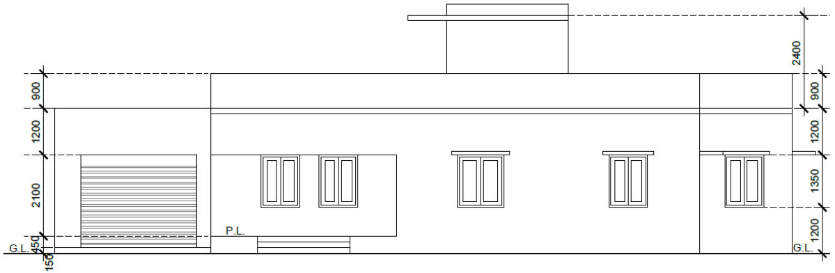
Fig 3.3 Elevation
