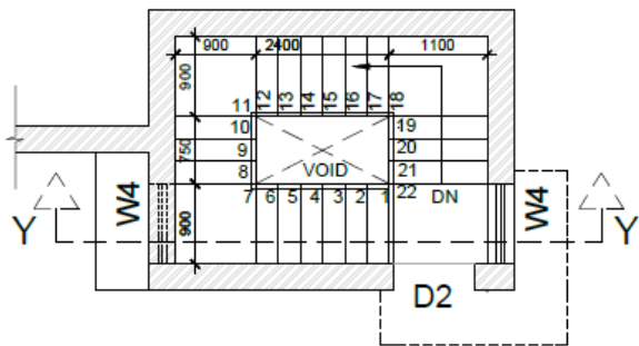
Fig 3.5 Plan and Section of a Residential Staircase
