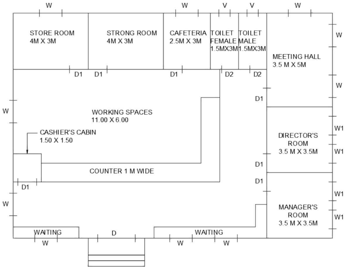
Fig 2.6.4: Line Plan of Bank
