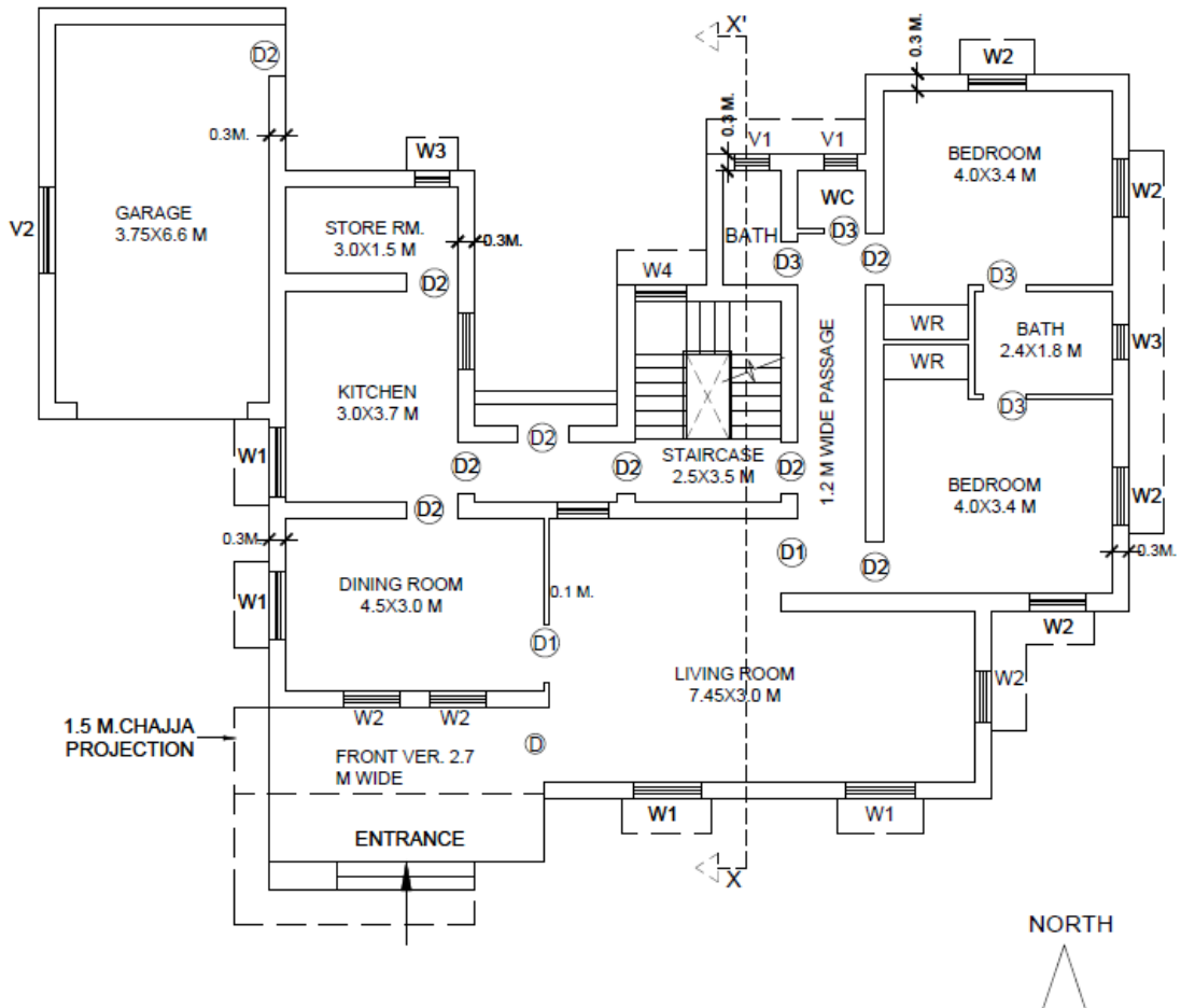
Fig 3.1 Plan
