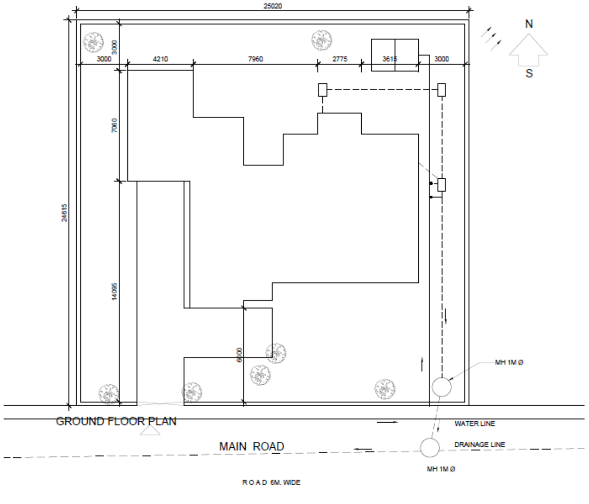
Fig 4.7 Site Plan
